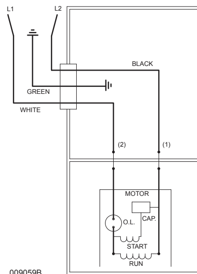
WIRING DIAGRAM FOR MODELS "N98-A", "N98-B", "N98-C" "E98-A", "E98-B" and "E98-C" 11/90 thru Current
